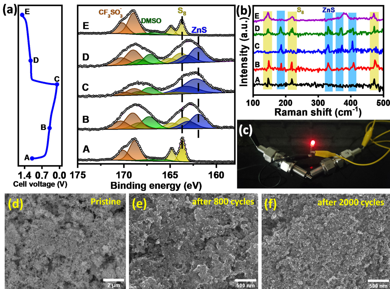
Fig. 5 (a) XPS and (b) Raman spectra of S@AC at different charge–discharge voltages; (c) photograph of an LED powered by assembling two Zn/ZnS batteries using the AZ/DMSO/ZnI 2 electrolyte; FESEM images of the sulfur cathode: (d) pristine, (e) after 800 cycles, and (f) after 2000 cycles.
