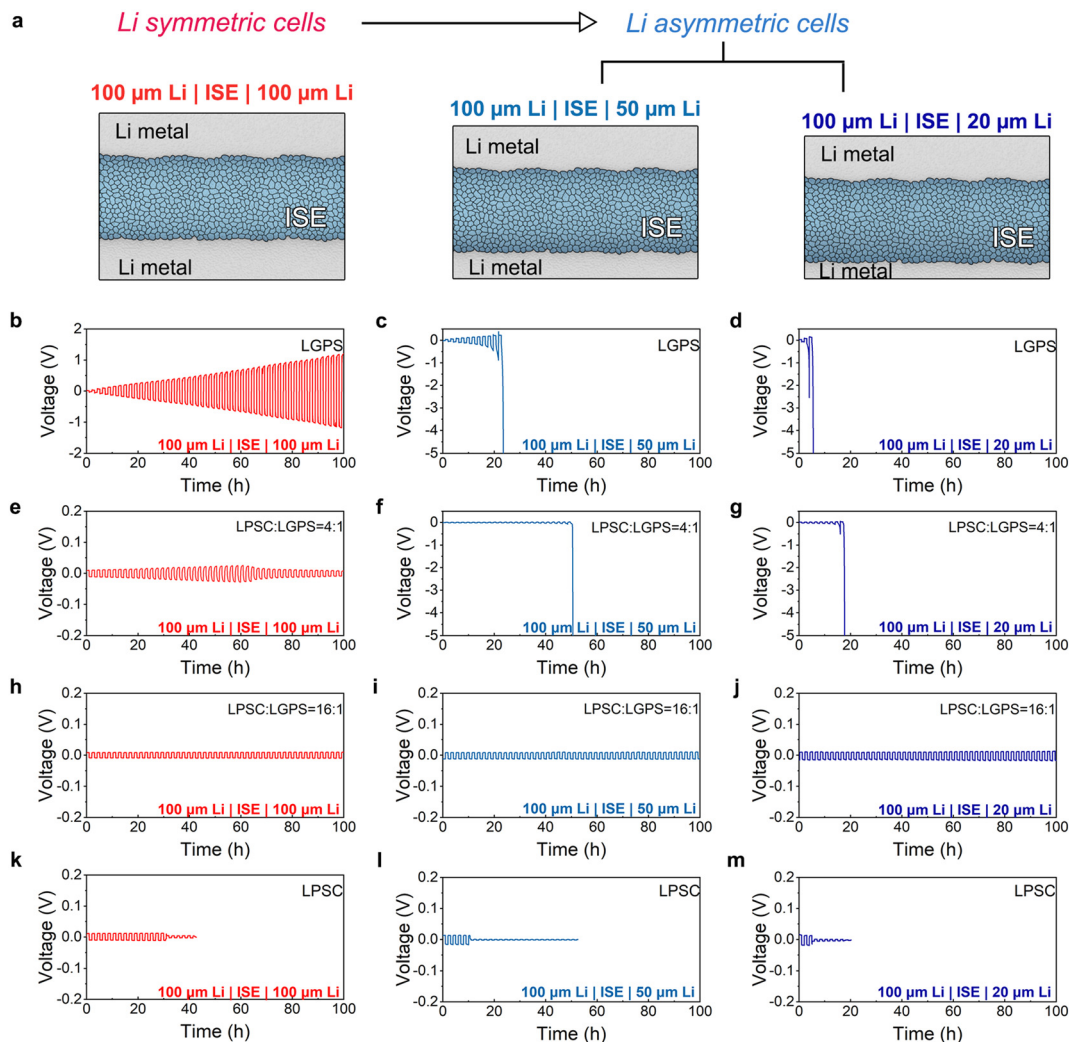
Fig. 2 (a) The schematic diagram of Li symmetric and asymmetric cells used in the evaluation. (b–d) Voltage profiles of the 100 \mu\text{m} thick Li|LGPS|100 \mu\text{m} thick Li symmetric cell (b), 100 \mu\text{m} thick Li|LGPS|50 \mu\text{m} thick Li (c) and 100 \mu\text{m} thick Li|LGPS|20 \mu\text{m} thick Li asymmetric cells (d). (e–g) Voltage profiles of the 100 \mu\text{m} thick Li|LPSC : LGPS = 4 : 1|100 \mu\text{m} thick Li symmetric cell (e), 100 \mu\text{m} thick Li|LPSC : LGPS = 4 : 1|50 \mu\text{m} thick Li (f) and 100 \mu\text{m} thick Li | LPSC : LGPS = 4 : 1|20 \mu\text{m} thick Li asymmetric cells (g). (h–j) Voltage profiles of the 100 \mu\text{m} thick Li|LPSC : LGPS = 16 : 1|100 \mu\text{m} thick Li symmetric cell (h), 100 \mu\text{m} thick Li|LPSC : LGPS = 16 : 1|50 \mu\text{m} thick Li (i) and 100 \mu\text{m} thick Li|LPSC : LGPS = 16 : 1|20 \mu\text{m} thick Li asymmetric cells (j). (k–m) Voltage profiles of the 100 \mu\text{m} -thick Li|LPSC|100 \mu\text{m} thick Li symmetric cell (k), 100 \mu\text{m} Li|LPSC|50 \mu\text{m} thick Li (l) and 100 \mu\text{m} thick Li|LPSC|20 \mu\text{m} thick Li asymmetric cells (m).
