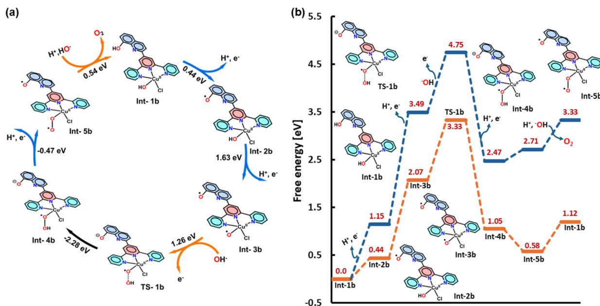
Fig. 12 (a) Catalytic cycle for the complete oxygen evolution reaction by catalyst b . (b) Energy profile diagram for catalyst b , where the blue path is shown without the pH correction factor and the orange path is shown with the pH correction factor at pH = 12 (all values are in eV).
