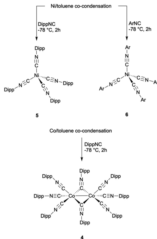
Scheme 2 Synthesis of cobalt and nickel complexes 4, 5, and 6.
