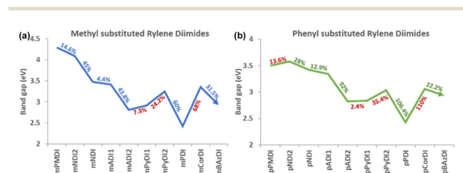
Fig. 5 Band gap trends of (a) methyl substituted and (b) phenyl substituted rylene diimides. A linear decrease in the bandgap with increasing rylene core is observed with two deviations: increasing band gap of PyDI and CorDI.
