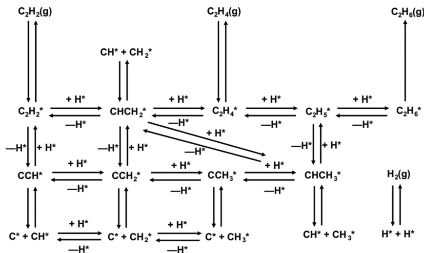
Fig. 1 Overall reaction network of C_2H_2 hydrogenation on Pd. Reproduced from literature 30 with permission. It includes adsorption reactions, desorption reactions, the main surface reactions and secondary surface reactions.
