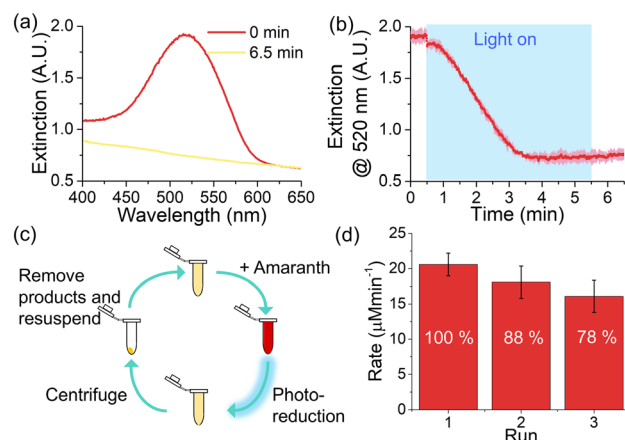
Fig. 3 (a) Extinction spectra of 0.5 \text{ mg mL}^{-1} Flap Mix and 50 \text{ }\mu\text{M} amaranth before and after light irradiation. (b) Extinction at 520 \text{ nm} over time during the photo-reduction of amaranth with Flap Mix . (c) Scheme showing the recycling of the photocatalyst and (d) the rate of amaranth photoreduction during each sequential run ( n = 3 ).
