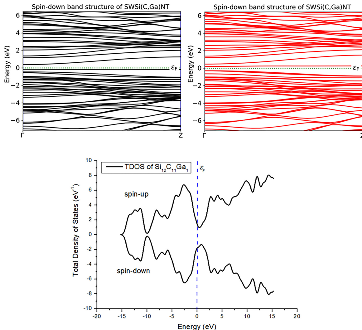
Fig. 9 The calculated spin-up (black) and spin-down (red) band structures, and TDOS diagram for \text{Si}_{12}\text{C}_{11}\text{Ga}_1 NTs.
