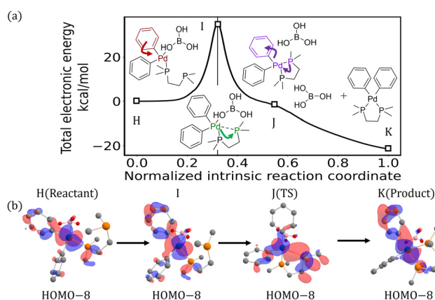
Fig. 6 Potential energy profile along the intrinsic reaction coordinate for the third-step transmetalation process in the oxo-palladium mechanism of the Suzuki–Miyaura cross-coupling reaction, accompanied by (a) the electron motion driving the reaction as revealed by ROET analysis, and (b) the corresponding changes in electron distribution of the identified reactive orbitals. In this process, the ancillary ligand returns to its bidentate coordination, and the boronic acid that was coordinated to the Pd center dissociates. Red–brown arrows indicate electron transfer in the early stage of the reaction, green arrows represent the middle stage, and purple arrows correspond to the late stage. The functional groups that play an active role in driving the electron motion at each reaction stage are highlighted in the corresponding colors. For a more detailed depiction of electron motions, refer to the attached animations.
