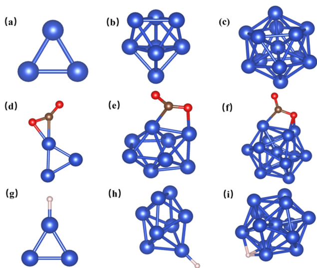
Fig. 1 (a)–(c) Structures of the pristine Cu 3 , Cu 8 and Cu 13 clusters. (d)–(f) The most stable adsorption configurations for CO 2 on Cu 3 , Cu 8 , and Cu 13 clusters. (g)–(i) The optimized configurations for H adsorption on Cu 3 , Cu 8 , and Cu 13 .
