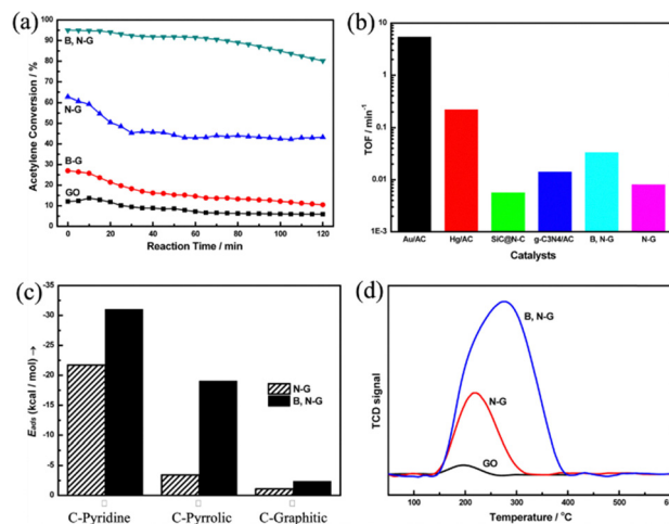
Fig. 10 (a) Catalytic reactivity evaluation of GO, B-G, N-G and B, N-G. The reactions were carried out at 150 °C, atmospheric pressure, a gas hourly space velocity (GHSV) of 36 h -1 , HCl/C_2H_2 = 1.15/1 (volume ratio). (b) The TOFs for different catalysts: Au/AC, Hg/AC, SiC@N-C, g-C 3 N 4 /AC, B, N-G, N-G. (c) E_{ads} of HCl on different types of active sites in N-G and B, N-G. C-pyridine: the carbon atoms bonded with pyridinic N species. C-pyrrolic: the carbon atoms bonded with pyrrolic N species. C-graphitic: the carbon atoms bonded with graphitic N species. (d) TPD profile of HCl on GO, N-G and B, N-G. 90 Reproduced from ref. 90 with permission from American Chemical Society. Copyright 2015.
