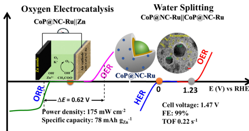
Fig. 15 Schematic illustration of bifunctional electrocatalytic performances of CoP@NC-Ru towards the ORR, OER, and HER. Adapted from ref. 105.
