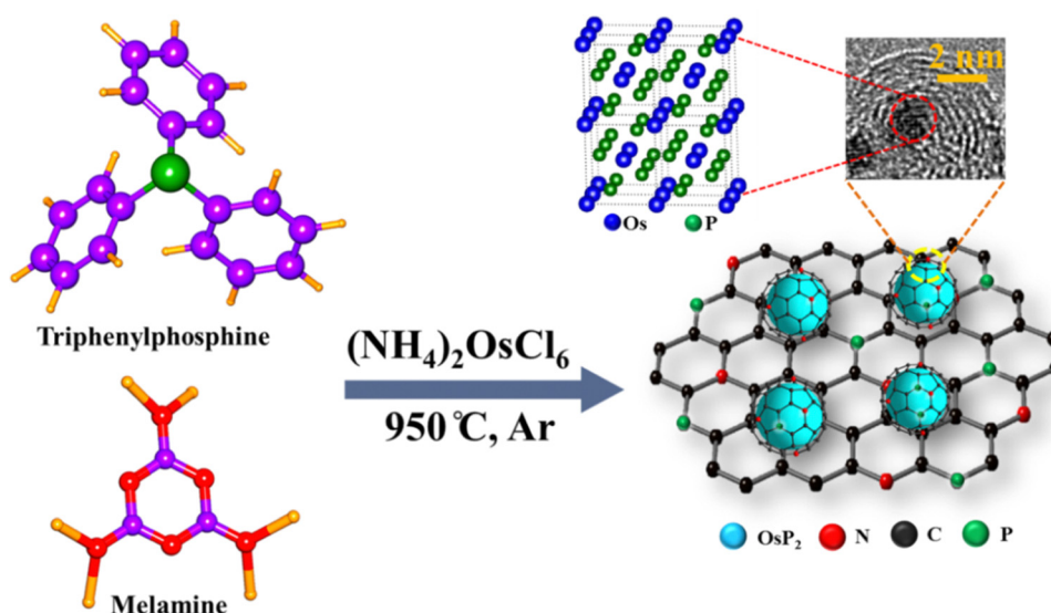
Fig. 5 Synthesis of \text{OsP}_2\text{@NPC} using TPP as a phosphidating agent. Reproduced with permission from ref. 65. Copyright 2019 Royal Society of Chemistry.
