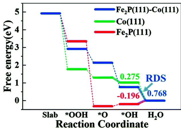
Fig. 14 The free energy diagram for Fe 2 P(111)-Co(111), Co(111), and Fe 2 P(111). Reproduced with permission from ref. 138. Copyright 2022 Royal Society of Chemistry.
