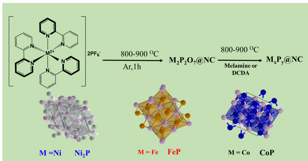
Fig. 4 Universal method for the synthesis of heteroatom-doped graphitic carbon encapsulated TMPs using a metal polypyridyl complex as a single source precursor. \text{Ni}_2\text{P@NC} , \text{FeP@NC} , and \text{CoP@NC} are synthesized using the corresponding polypyridyl complexes.
