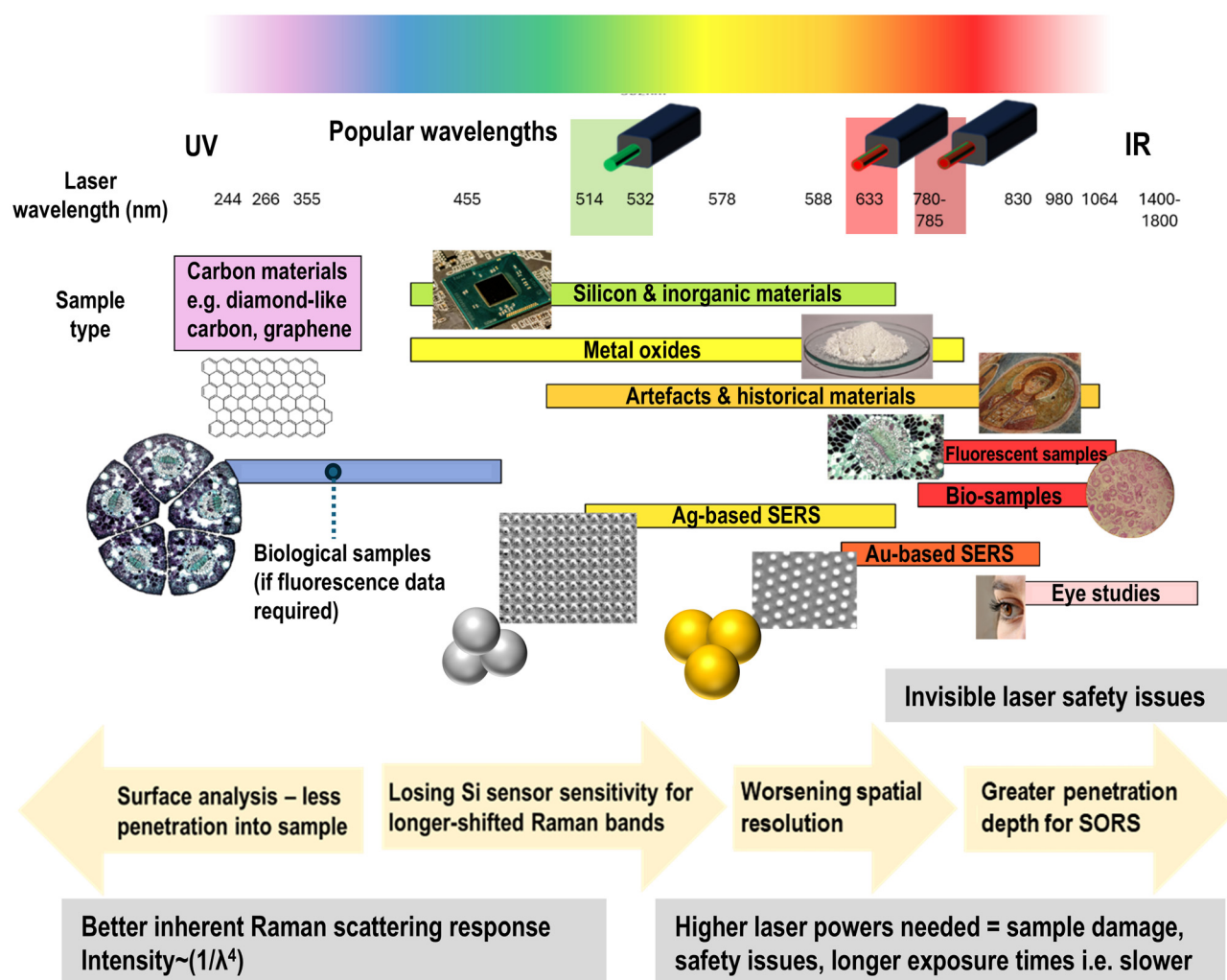
Fig. 4 Recommendation of wavelengths with respect to the desired sample types. Images reprinted with permission under CC-BY-4.0, details in ESI.†
