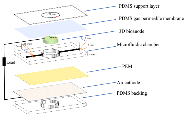
Figure 3. Layer-by-layer design for 3D Bio-anode Embedded BPV Cell Unit.
