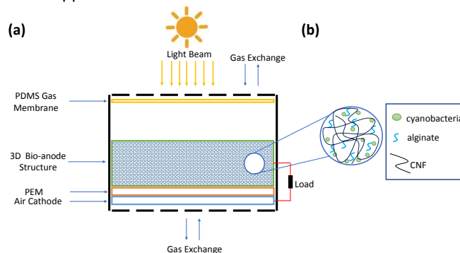
Figure 1. Schematic of 3D hydrogel-based bio-anode embedded BPV cell unit for energy harvesting. (a) Schematic of 3D hydrogel-based bio-anode embedded BPV cell unit (b) Components of the 3D hydrogel-based bio-anode structure.
