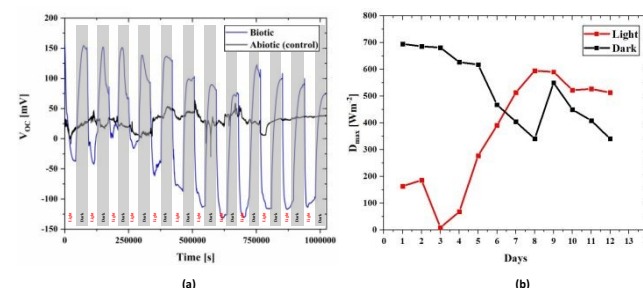
Figure 4. Long-term open circuit voltage results of the scaffold with bacteria and without bacteria under 12 hours of light, provided by a 16.7 W.m -2 white light source, and 12 hours of dark conditions. (a) The graph demonstrates two different measurement results; the black line indicates the open circuit voltage measurement result of the empty scaffold structure without bacteria (with a platinum wire anode and an air cathode). The cyclic blue curve shows the open circuit voltage measurement result of the bacterial scaffold (with a platinum wire anode and an air cathode). (b) Observation of the change in maximum power densities of the biotic scaffold over time under light and dark conditions.
