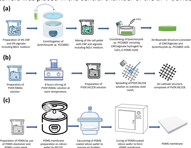
Figure 2. The fabrication process of (a) 3D-Bioanode composed of CNF/Alginate and Synechocystis sp. PCC 6803. (b) air-cathode consisting of PVDF/AC/CB. (c) PDMS membrane.
