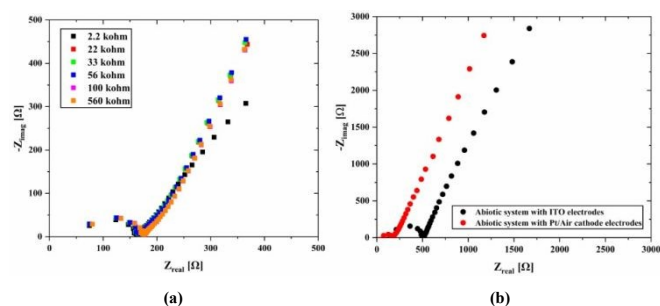
Figure 6. Comparison of EIS measurements of abiotic systems. (a) The results of the tests performed with the scanning EIS technique using the Pt/Air cathode electrode system in the abiotic system. In this part, resistors of 2.2 k \Omega , 22 k \Omega , 33 k \Omega , 56 k \Omega , 100 k \Omega , and 560 k \Omega were used, respectively. (b) Impedance measurements with the open circuit method using Pt/Air cathode and ITO/ITO electrodes in the abiotic system and comparison of the results.
