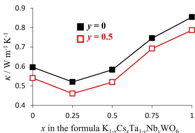
Fig. 14 The compositional dependence of the thermal conductivity of K_{1-x}Cs_xTa_{1-y}Nb_yWO_6 ( 0 \leq x \leq 1 ; y = 0, 0.5 ) at 300^\circ\text{C} .
