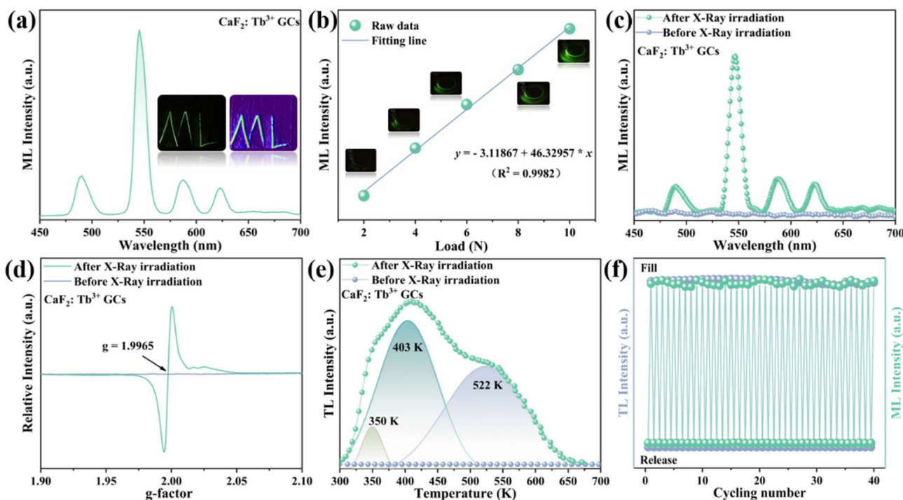
Fig. 2 (a) ML spectrum of the \text{CaF}_2\text{: Tb}^{3+} GCs (the illustrations show an ML visualization of a handwriting trajectory through long exposure and extracted dimensional color maps from the corresponding photos). (b) The relationship between ML intensity of \text{CaF}_2\text{: Tb}^{3+} GCs and applied load (insets show the corresponding ML photographs). (c) ML spectra of \text{CaF}_2\text{: Tb}^{3+} GCs before and after X-ray pre-irradiation. (d) EPR spectra before and after X-ray pre-irradiation of \text{CaF}_2\text{: Tb}^{3+} GCs. (e) TL curves and Gaussian fitted result of \text{CaF}_2\text{: Tb}^{3+} GCs before and after X-ray pre-irradiation. (f) Cycling stability of ML/TL in \text{CaF}_2\text{: Tb}^{3+} GCs.
