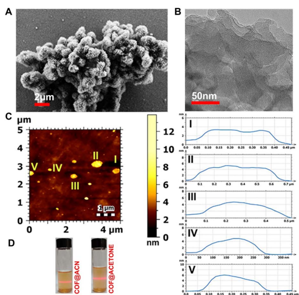
Fig. 3 (A) FESEM image of 1 showing the cotton-ball like morphology with small spikes on it. (B) HRTEM image of 1 showing a flake kind of structure. The inset showing the lattice fringes having an inter planar distance of 0.26 nm which is very close to the interlayer distance obtained from the structural model. (C) (Top) AFM image of 1 showing its nanosheet character. (Bottom) 1 dispersed in different solvents showing the Tyndall effect for a prolonged time. (D) The height profile plot shows the thickness of the nanosheets to be in the range of \approx 4 –6 nm (see the ESI† for more images).
