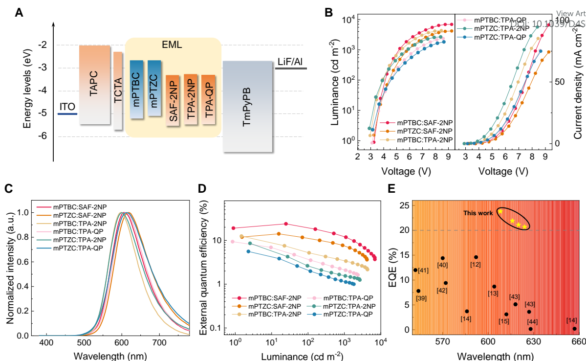
Figure 5. (A) Device configuration of the exciplex-based OLEDs. Luminance-voltage-current density curves (B), EL spectra (C) and EQE-luminance plot (D) of mPTBC:SAF-2NP, mPTBC:TPA-QP, mPTZC:SAF-2NP, mPTZC:TPA-2NP and mPTZC:TPA-QP. (E) EQE vs. wavelength plot of representative yellow to deep-red OLEDs based on exciplex emitters.
