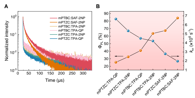
Figure 4. (A) PL decay curves of mPTBC:SAF-2NP, mPTZC:SAF-2NP, mPTBC:TPA-2NP, mPTBC:TPA-QP, mPTZC:TPA-2NP and mPTZC:TPA-QP. (B) Variation trends of \Phi_{\text{PL}} and k_{\text{nr}} from mPTZC:TPA-QP to mPTBC:SAF-2NP (D:A = 9:1).
