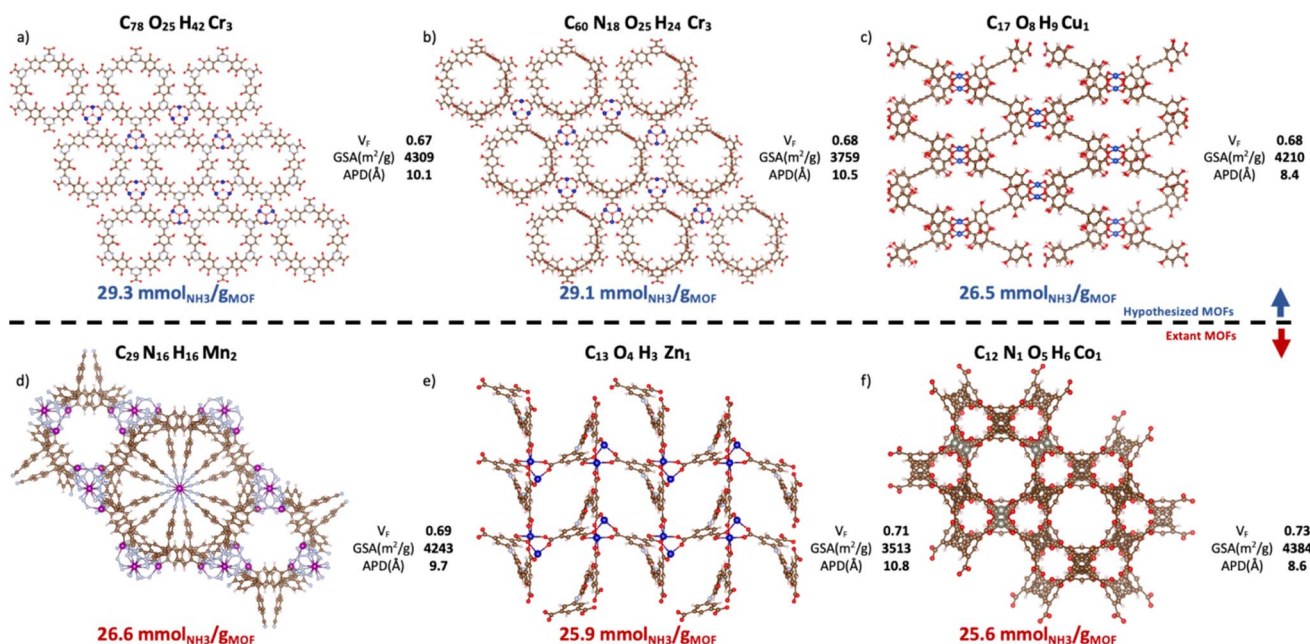
Fig. 10 Top-6 MOFs ranked by \Delta N_{\text{NH}_3} value. Hypothesized (a–c) and extant MOFs (d–f) are in the top and bottom rows, respectively. V_p , GSA, and APD represent, respectively, the void fraction, gravimetric surface areas, and average pore diameter from pore size distribution. The CSD refcode and corresponding publication can be found in Table S5 † with (a) n = 1 , (b) n = 2 , (c) n = 4 , (d) n = 3 , (e) n = 5 , (f) n = 6 , where n is the MOF ranking. The three hypothesized MOFs are potentially synthesizable per the free energy criterion by Anderson and Gómez-Gualdrón (Table S6 † ). 100 Ca MOFs appear in the top-14 but not in top-6 presumably due to suboptimal textural properties.
