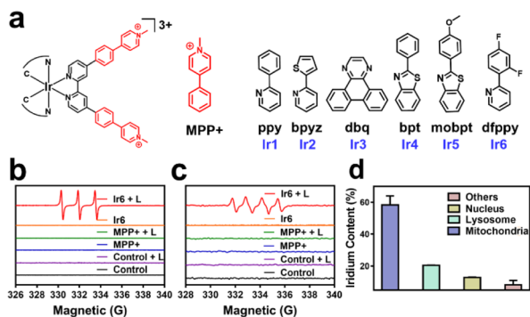
Fig. 1 (a) Chemical structures of the Ir(III) photosensitizers Ir1–Ir6 and MPP+. (b) Electron spin resonance spectra of Ir6 and MPP+ upon incubation with the 1 O 2 -specific scavenger 2,2,6,6-tetramethylpiperidine in the dark or upon light irradiation (L). (c) Electron spin resonance spectra of Ir6 and MPP+ upon incubation with the scavenger 5,5-dimethyl-1-pyrroline-N-oxide in the dark or upon light irradiation (L). (d) The subcellular distribution of A375 cells upon incubation with Ir6 (10 μM) for 6 h to determine the metal content inside the major organelles. L = two-photon laser irradiation at 720 nm, 40 mW, 120 s.
