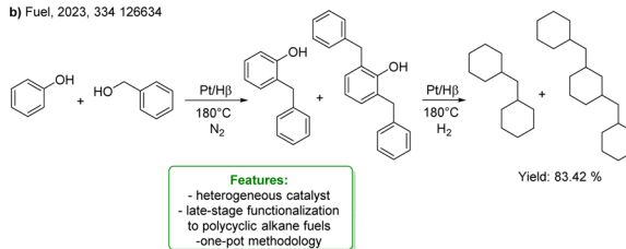
Scheme 28 Acid-catalysed alkylation of phenol, and subsequent HDO to obtain bi- or poly-cycloalkanes or high-density biofuels (a) two-step synthesis of perhydrofluorene, from phenols and benzyl acetate catalysed by solid acid montmorillonite (MMT), and Pd/C. 98 (b) One-pot strategy for preparing polycyclic alkane from phenol and benzyl alcohol over a bifunctional Pt/H \beta catalyst. 99
