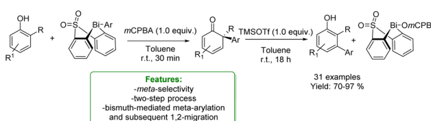
Scheme 80 Arylation of phenols with modular bismacycles. (a) Ortho -arylation of phenols with modular bismacycles. 218 (b) Meta -arylation of phenols with modular bismacycles. 219
