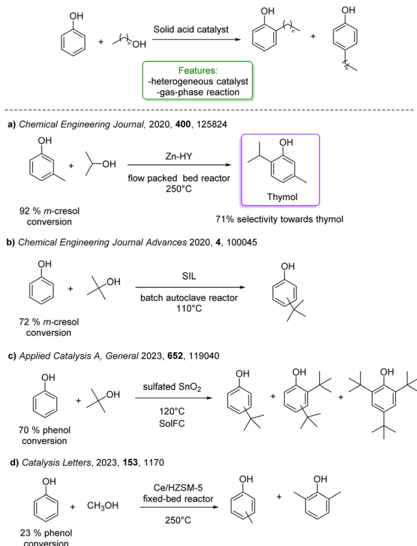
Scheme 27 Solid acid catalysed ortho -alkylation of phenols with simple and short alcohols. (a) Alkylation of phenol with n PrOH Zn-HY modified zeolite catalysts. 94 (b) Alkylation of phenol with t BuOH supported ionic liquid catalysts. 95 (c) Alkylation of phenol with t BuOH metal oxide catalysts (SnO 2 , TiO 2 and ZrO 2 ). 96 (d) Alkylation of phenol with methanol catalysed by Ce/HZSM-5. 97
