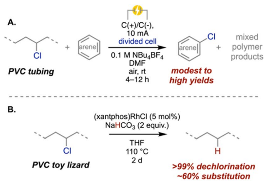
Scheme 6 (A) PVC as a chlorine source for organic synthesis using electrochemistry. 118 (B) Reductive hydrodechlorination using a metal catalyst and a hydride source. 66
