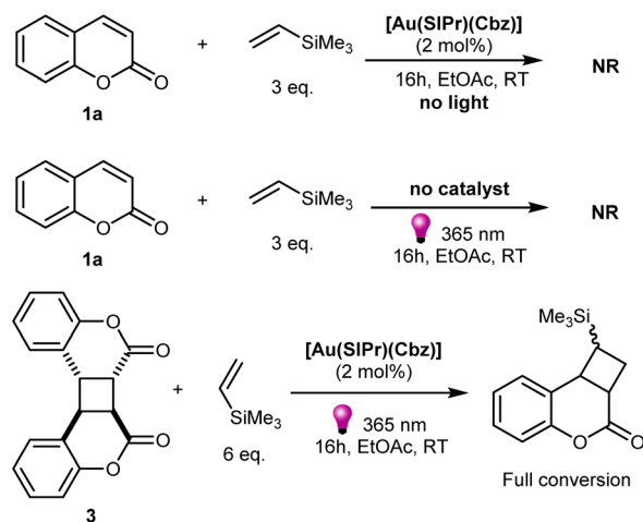
Scheme 4 Control experiments.
