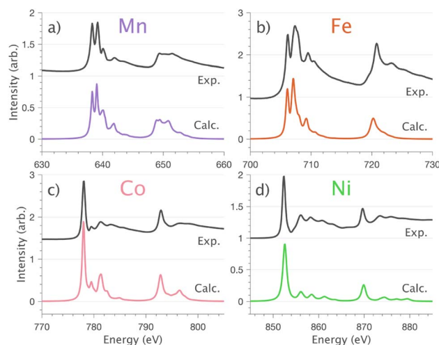
Fig. 7 Normal incidence ( \vec{E} \perp c ) single crystal \text{L}_{2,3} -edge XAS measurements and calculations for \text{Li}_2(\text{Li}_{1-x}\text{TM}_x)\text{N} (where \text{TM} = (a) Mn, (b) Fe, (c) Co and (d) Ni). Experimental spectra measured at 21 K (black) and optimised charge-transfer multiplet calculations (colour).
