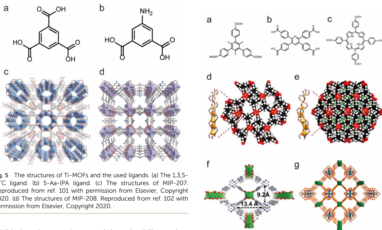
Fig. 6 The structures of representative In(III) -MOFs and the used ligands. (a) The H_3CTTA ligand. (b) The H_4TCP ligand. (c) The H_2TCP ligand. (d) BUT-172. Reproduced from ref. 103 with permission from the Royal Society of Chemistry, Copyright 2020. (e) BUT-173. Reproduced from ref. 103 with permission from the Royal Society of Chemistry, Copyright 2020. (f) In(tcp) . Reproduced from ref. 104 with permission from the Royal Society of Chemistry, Copyright 2021. (g) USTC-8. Reproduced from ref. 105 with permission from the American Chemical Society, Copyright 2018.
