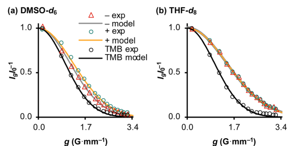
Fig. 2 Diffusion profiles of \text{Ph}_3\text{SiF}_2^- ("–"), ^n\text{Bu}_4\text{N}^+ ("+") and the internal diffusion standard ("TMB") in: (a) 1.5 mM TBAT and 263 mM TMB in DMSO- d_6 , and (b) 207 mM TBAT and 252 mM TMB in THF- d_8 ; both at 300 K.
