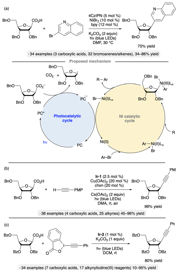
Scheme 16 Photocatalytic, decarboxylative couplings of glycosyl-1-carboxylates with (a) bromoarenes; 51 (b) alkynes; 53 and (c) alkynyl iodide(III) reagents. 54 bpy denotes 2,2'-bipyridine; Ir-1 denotes [Ir(dF(CF 3 )ppy) 2 (dtbbpy)]PF 6 ; chxn denotes trans -1,2-diaminocyclohexane; Ir-2 denotes [Ir(dF(CF 3 )ppy) 2 (d(CF 3 )bpy)]PF 6 .
