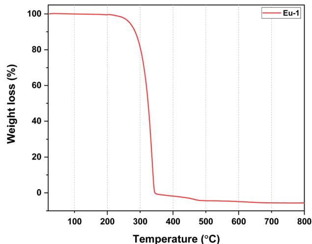
Fig. 1 TGA profile of Eu-1 between 25 and 800 °C under \text{N}_2 atmosphere.
