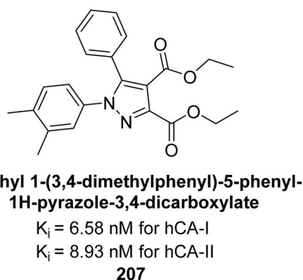
Fig. 73 Chemical structures of compounds 206 and 207; their K_i values against hCA-I and II along with docking images of compound 206 and 207.
