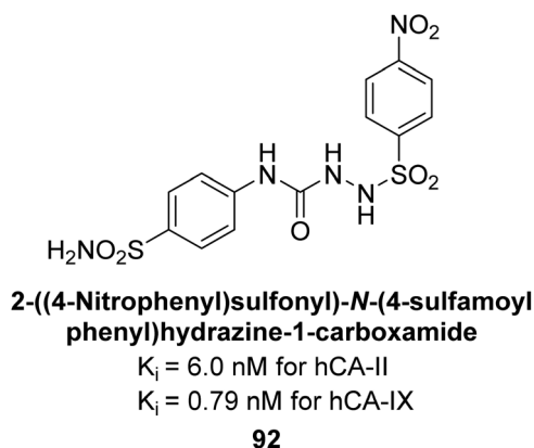
Fig. 36 Chemical structure of compound 92 and their K_i values against hCA-II and IX.
