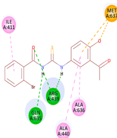
Fig. 69 Acetylphenol-based acyl thioureas and interaction of compound 142f with various amino acid residues.
