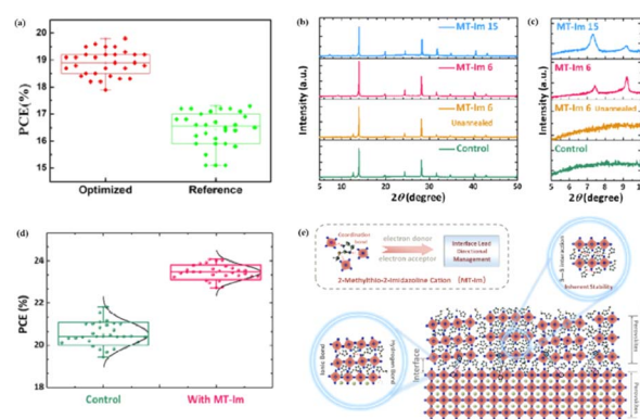
Fig. 12 Box charts of (a) PCE of optimized TEPA-MAPbI 3–x Cl x and reference MAPbI 3–x Cl x -based devices. Adapted with permission from ref. 139. Copyright 2020 American Chemical Society. (b and c) XRD patterns of the control, unannealed MT-Im (6 mg mL -1 ), and MT-Im (15 mg mL -1 ) perovskite films. (d) PCE distributions for the control and MT-Im perovskite devices. (e) Schematic illustration of the effective management by inherently stable MT-Im LDP for the Pb-based defects at the interface. Adapted with permission from ref. 87. Copyright 2020 American Chemical Society.
