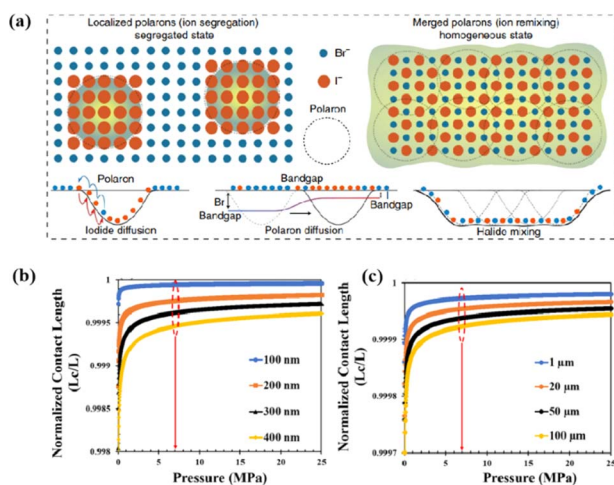
Fig. 32 (a) Illustration of halide ion distribution for a MAPb(Br 0.8 I 0.2 ) 3 perovskite lattice in response to low carrier density (left) and high carrier density (right). Adapted with permission from ref. 209. Copyright 2020 Springer Nature. Analytical model prediction of pressure effects on contact length ratios: (b) effects of pressure on the surface contacts for different thicknesses of the films (for particle size of 1 μm) and (c) effects of pressure on surface contacts for different sizes of the particles (for a film thickness of 250 nm). Adapted with permission from ref. 31. Copyright 2020 Springer Nature.
