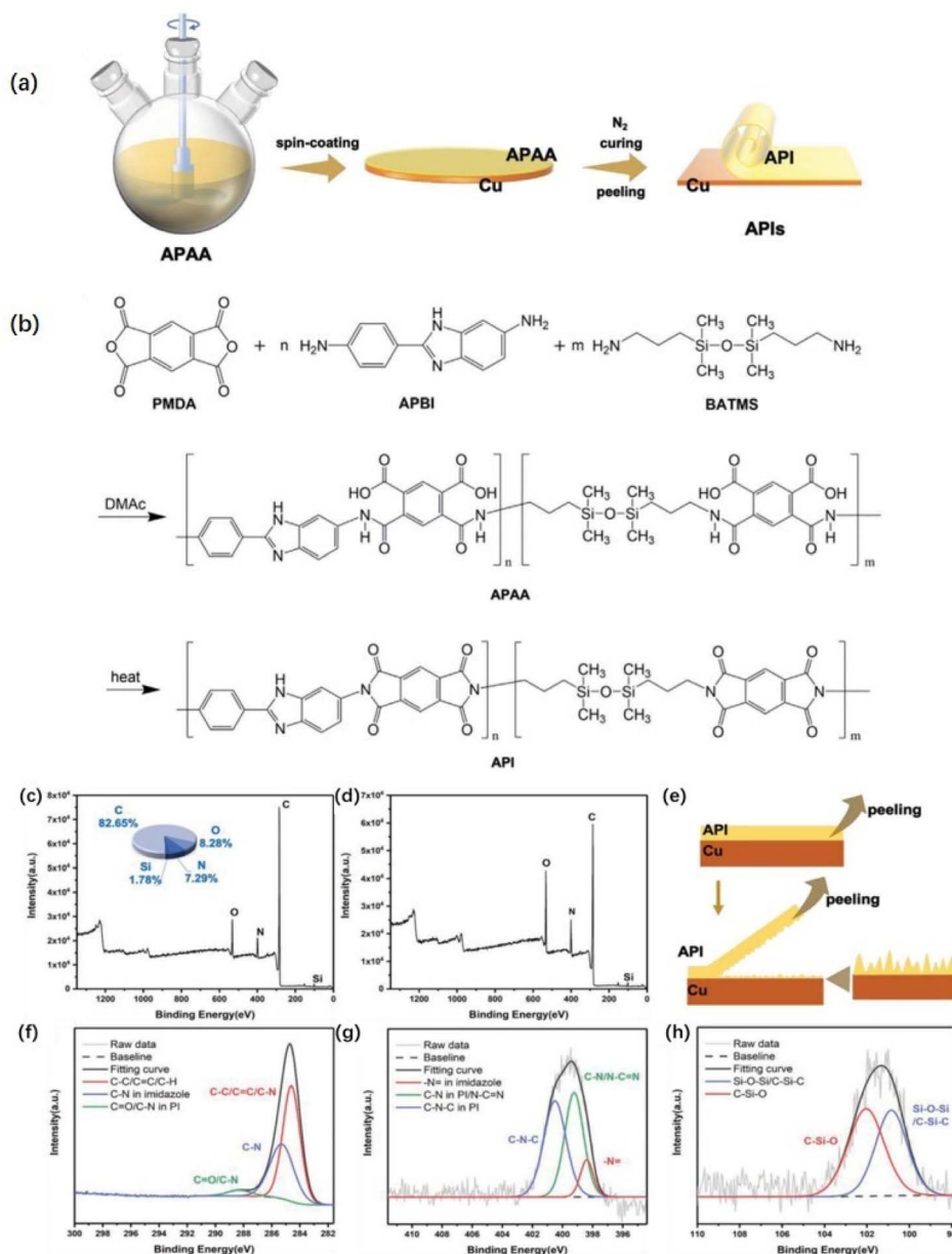
Fig. 6 (a) Schematic of the synthesis procedure of adhesive polyimide (API), and (b) the reaction principle of API precursor solution (APAA) and API; XPS full (wide-scan) spectra (the illustration shows the element-content distribution) of (c) copper surface and (d) API-2 surface after peeling test; (e) schematic of the peeling process showing the principle of adhesion; (f) C 1s, (g) N 1s, and (h) Si 2p peaks of copper surface after peeling test by XPS. Adapted from ref. 101 with permission from Advanced Materials Interfaces , Copyright 2022.
