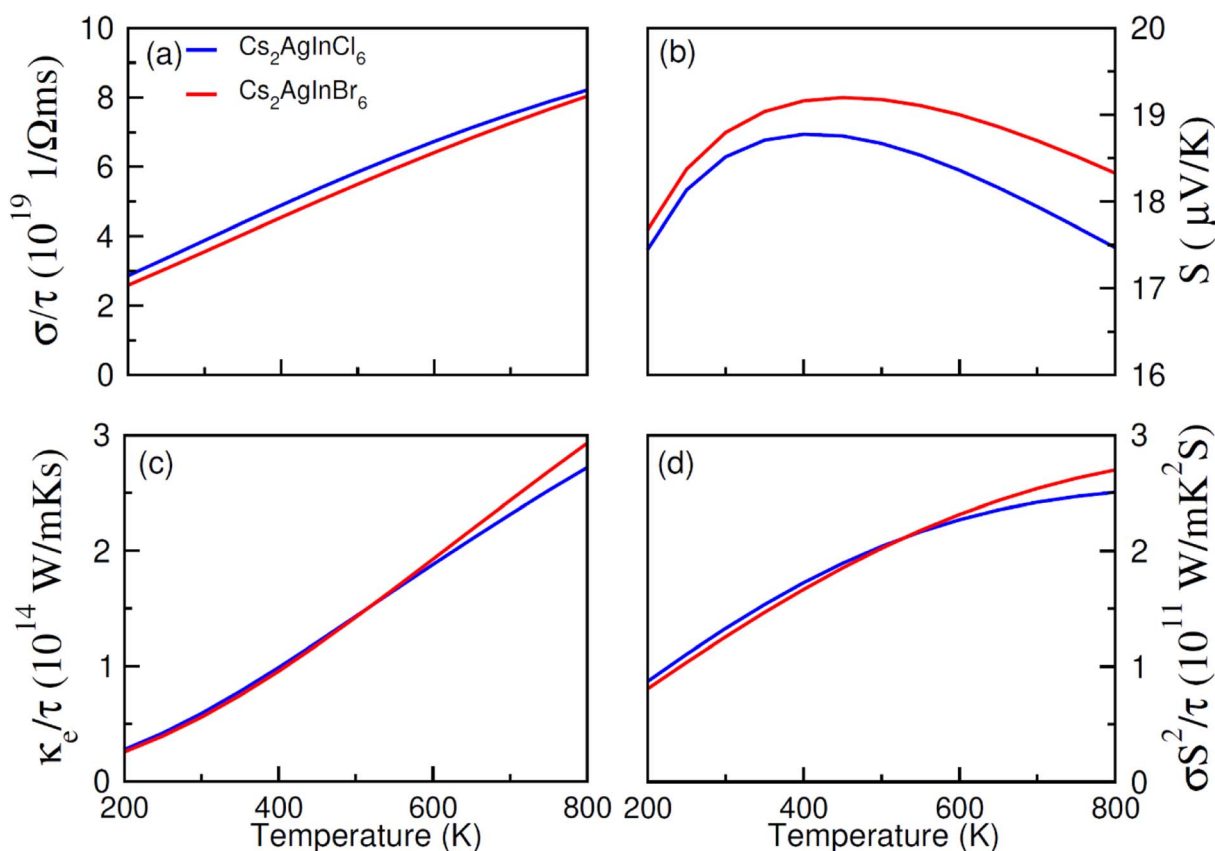
Fig. 8 The calculated (a) electrical ( \sigma/\tau ), (b) Seebeck coefficient ( S ), (c) thermal ( \kappa_e/\tau ) conductivities, (d) and power factor for NM \text{Cs}_2\text{AgInCl/Br}_6 against temperatures (200 K–800 K).
