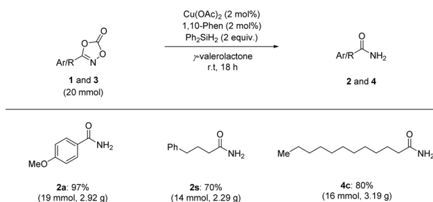
Scheme 4 Gram-scale synthesis of primary amides 2 and 4.
