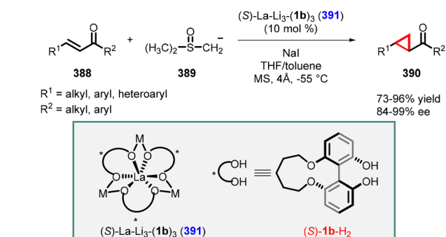
Scheme 86 La-Li 3 -(biphenyldiolate) 3 /NaI complex catalyzed MIRC cyclopropanation of enones with dimethyloxosulfonium methylide.
