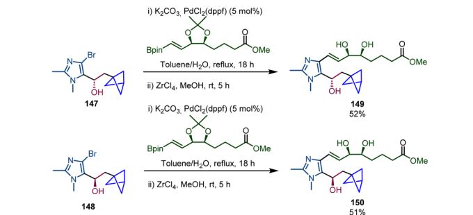
Scheme 26 Synthesis of \beta -chiral BCPs 149 and 150 as analogues of lipoxin \text{A}_4 .
