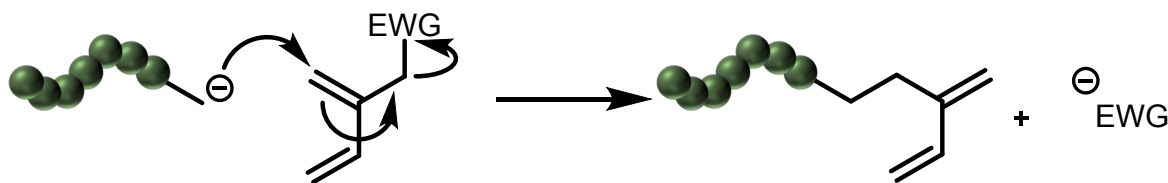
Scheme 3: Proposed mechanism of the backside-collapse, as described in the works of Takenaka et al. 100,101 View Article Online DOI: 10.1039/D4PY00805G
