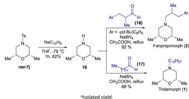
a Isolated yield.
