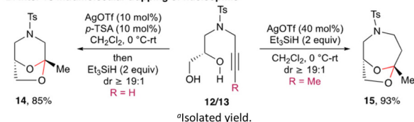
a Isolated yield.
