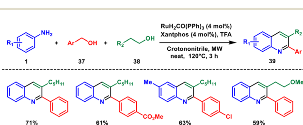
Scheme 14 Ru-catalysed reaction with alkyl and aryl alcohol.
