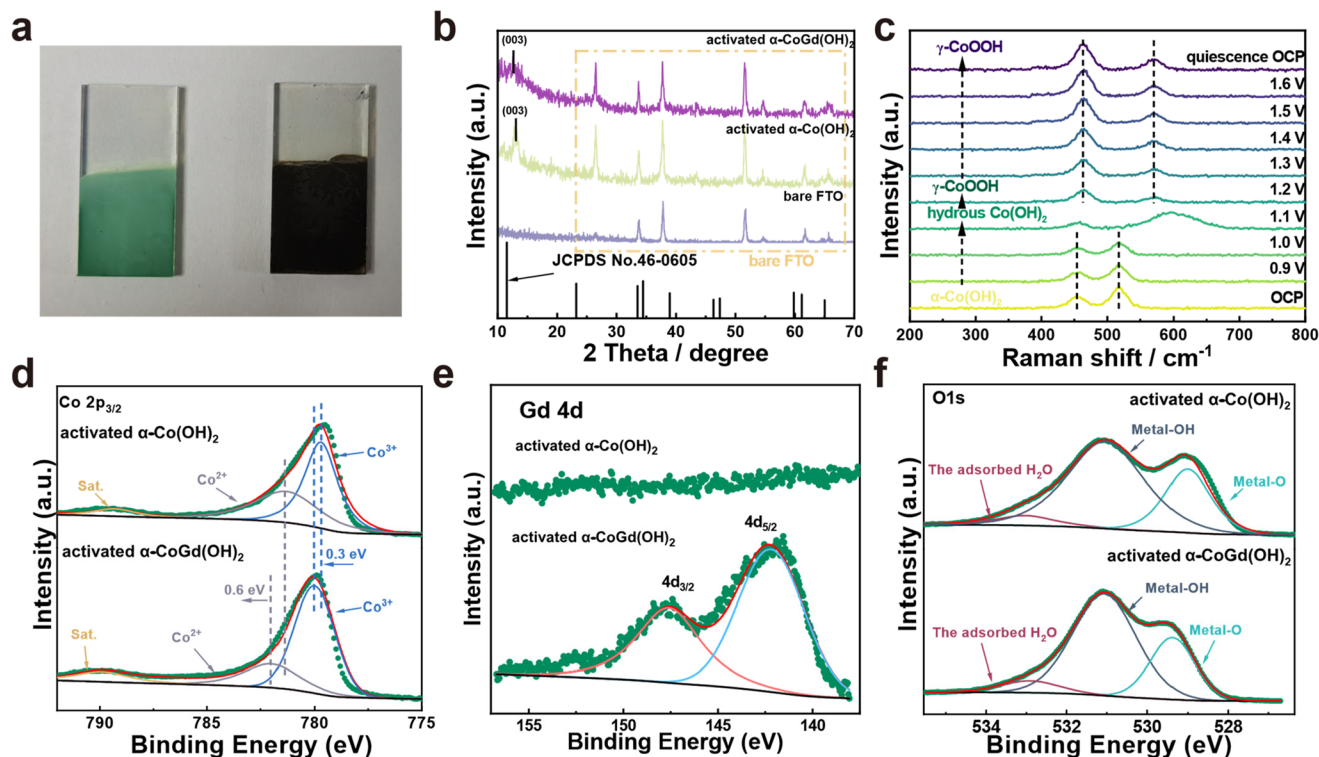
Fig. 3 (a) The optical images of \alpha -CoGd(OH) _2 before and after activation. (b) The powder XRD patterns of activated \alpha -CoGd(OH) _2 and \alpha -Co(OH) _2 . Herein, the XRD pattern of bare FTO was used as a reference. (c) In situ Raman spectra of activated \alpha -CoGd(OH) _2 at 0.9–1.6 V vs. RHE, as well as the ex situ ones at the OCP. (d) Co 2p _{3/2} XPS spectra of \alpha -CoGd(OH) _2 and \alpha -Co(OH) _2 after activation. (e) The Gd 4d XPS spectrum of \alpha -CoGd(OH) _2 after activation. (f) The O 1s XPS spectra of \alpha -CoGd(OH) _2 and \alpha -Co(OH) _2 after activation.
