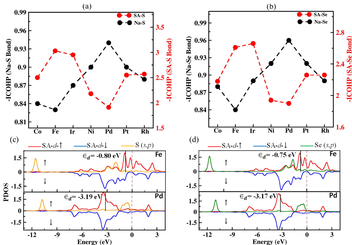
Fig. 6 The strength of (a) \text{Na-S} and \text{SA-S} bonds and (b) \text{Na-Se} and \text{SA-Se} evaluated using the integrated COHP ( -\text{ICOHP} ) for the \text{Na}_2\text{X-SAC} system. (Here, the depicted bond strength ( -\text{ICOHP} ) is the sum of the spin-up and spin-down -\text{ICOHP} values in eV per bond.) (c and d) The calculated partial density of states (PDOS) of \text{Na}_2\text{X-SAC} ( \text{SAC} = \text{Fe}, \text{Pd} ) systems. The up-spin d-band center values are illustrated on the PDOS plot, measured with respect to the Fermi level set at zero.
