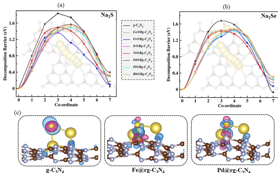
Fig. 5 Decomposition paths and decomposition energies of (a) \text{Na}_2\text{S} and (b) \text{Na}_2\text{Se} on the pristine \text{g-C}_3\text{N}_4 and \text{SA@rg-C}_3\text{N}_4 monolayers. (c) The charge density differences of \text{Na}_2\text{S} adsorbed on the pristine \text{g-C}_3\text{N}_4 and \text{SA@rg-C}_3\text{N}_4 monolayer. The blue regions represent electron accumulation, and magenta regions represent depletion.
