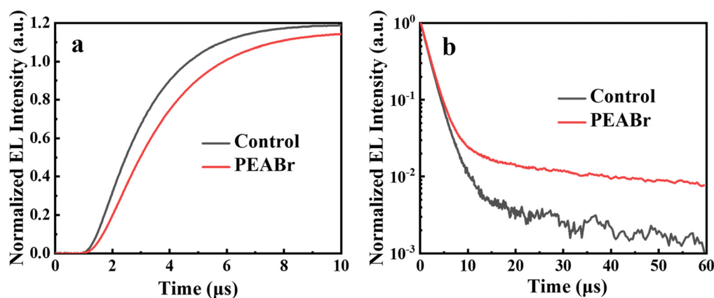
Fig. 3 (a) The rising part, and (b) the decayed part of TREL at a pulsed voltage of 3 V.
