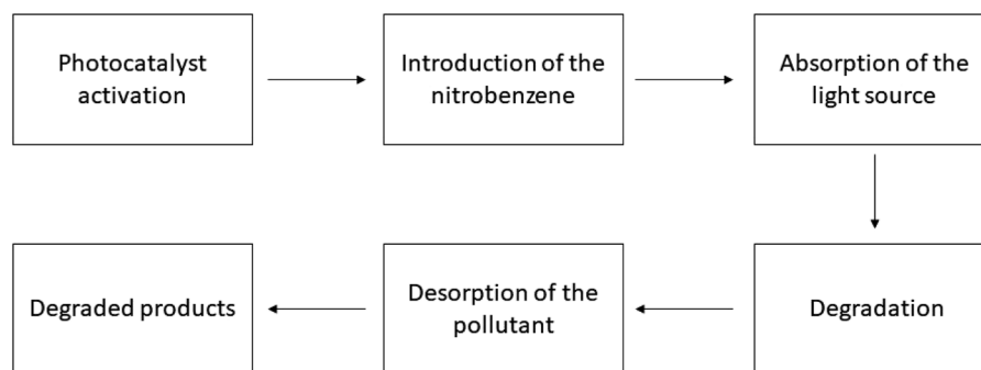
Fig. 4 Working procedure of the photocatalysts for nitrobenzene degradation.
