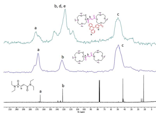
Fig. 4 ^{13}\text{C} NMR spectra of film 1-PTH (top), film 1 (middle) and N 1 , N 2 , N 4 , N 4 -tetraethylfumaramide (bottom).
