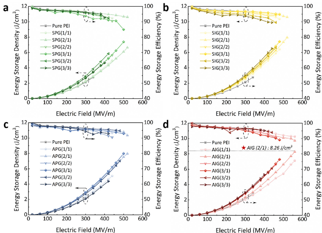
Fig. 4 The energy storage density and efficiency as a function of the electric field of (a) SPG, (b) SIG, (c) APG, and (d) AIG composite dielectrics.
