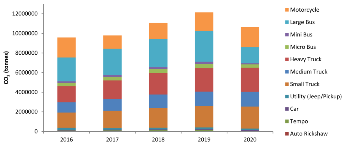
Fig. 2 Vehicular emission inventories of CO 2 from the year 2016 to 2020 in Bangladesh.
