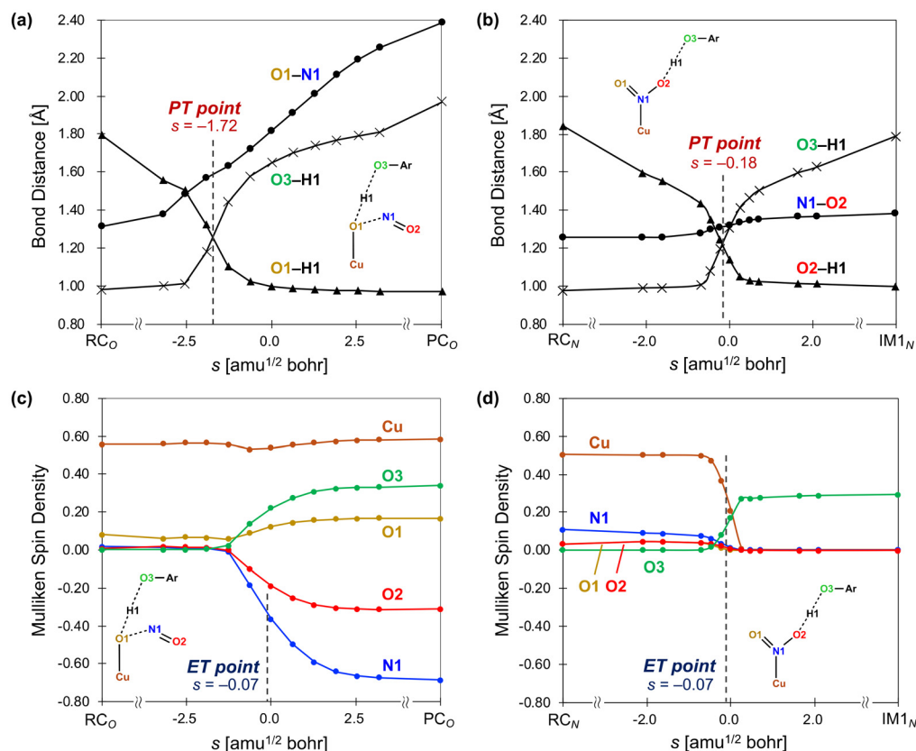
Fig. 4 Intrinsic coordinate plots of the changes in structures and spin densities from RC_O to PC_O via TS_O in the nitrite pathway (a and c) and from RC_N to IM1_N via TS1_N in the nitro pathway (b and d) as a function of the reaction coordinate s [amu 1/2 bohr]. The transition state is s = 0.0 . The proton transfer (PT) point is defined as the intersection between the two O-H distances (O1-H1 and O3-H1 in (a) and O2-H1 and O3-H1 in (b)). The electron transfer (ET) point is defined as the point where the spin density for the N1 (Cu) atom reaches the midpoint of RC_O and PC_O in (c) ( RC_N and IM1_N in (d)). Reproduced from ref. 37 with permission from the American Chemical Society, copyright 2023.
