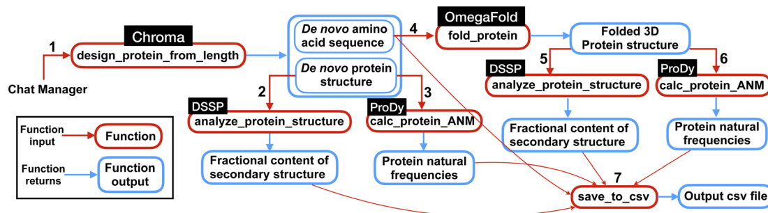
Fig. 3 Overview of the multi-agent work to solve the complex task posed in Experiment II, Section 2.2. First the multi-agent uses Chroma to generate de novo protein sequences and then computes natural frequencies and secondary structures content for the generated structures. Next, from de novo AA sequences, the model finds the 3D folded structures using OmegaFold and finally computes the frequencies and secondary structure content for the protein structures. Finally, the results are saved in a csv file as shown in Table 3. The numbers represent the sequence in which the functions are executed within the workflow.
