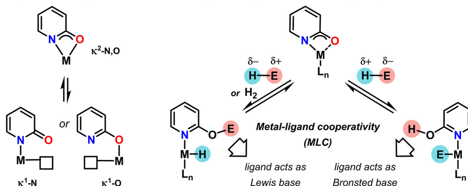
Scheme 1 Coordination bonding motifs of the 2-pyridone/2-pyridonate ligand platform.
