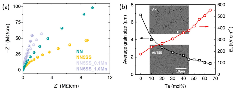
Fig. 21 (a) Nyquist-plot of the NN, NN-5SrSnO 3 , NN-5SrSnO 3 -0.1Mn, and NN-5 SrSnO 3 -1.0Mn samples. 49 (b) The composition dependence of average grain size and E_0 , the insets give the SEM micrographs of the AN and AN-Ta 0.55 ceramics, respectively. 77 Reprinted with permission ref. 49 from under the terms of the Creative Commons CC BY license, Springer Nature. Reprinted with permission from ref. 77, under the terms of the Creative Commons CC BY license, Springer Nature.
